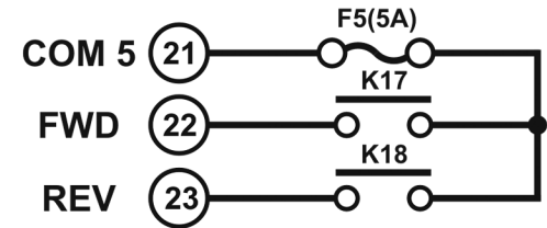
Push button 9~10
