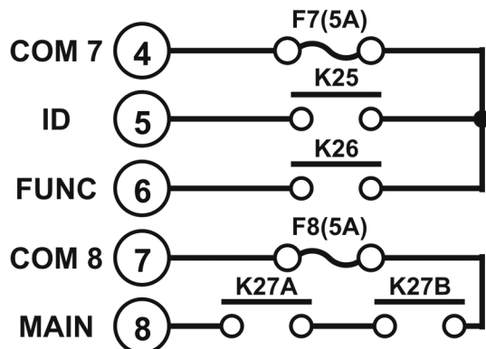
MAIN/ID/Function
