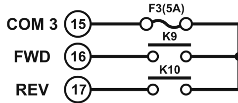
Push button 5~6
