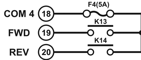
Push button 7~8
